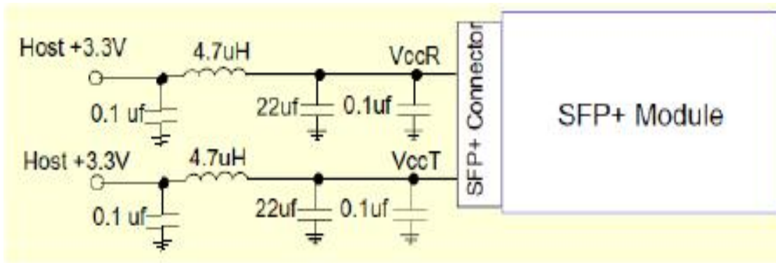
Recommended Host Board Power Supply Circuit
