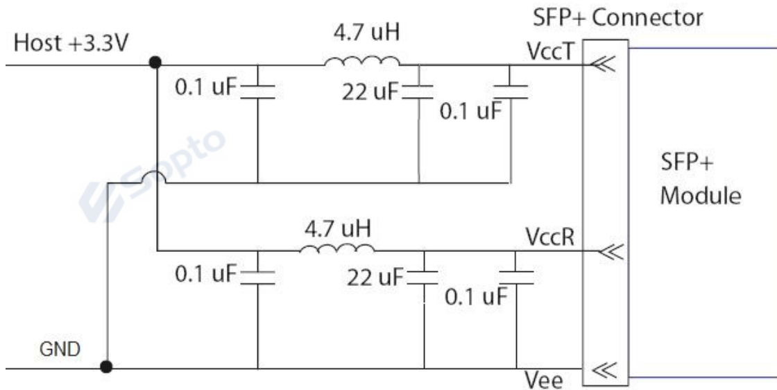
Recommended Host Board Power Supply Circuit
