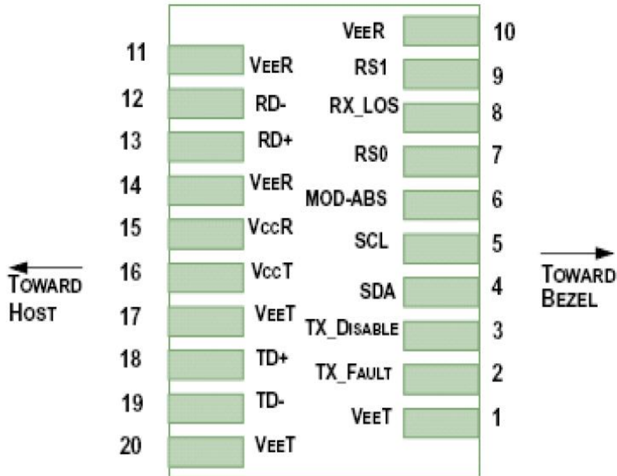
Figure1.Elecctrical Pin-out Details
