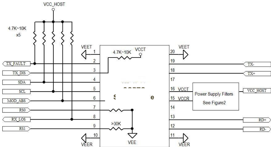
Figure4. Host-Module Interface
