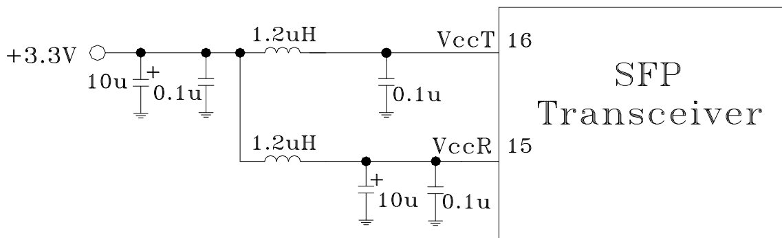
Recommended Host Board Power Supply Circuit
