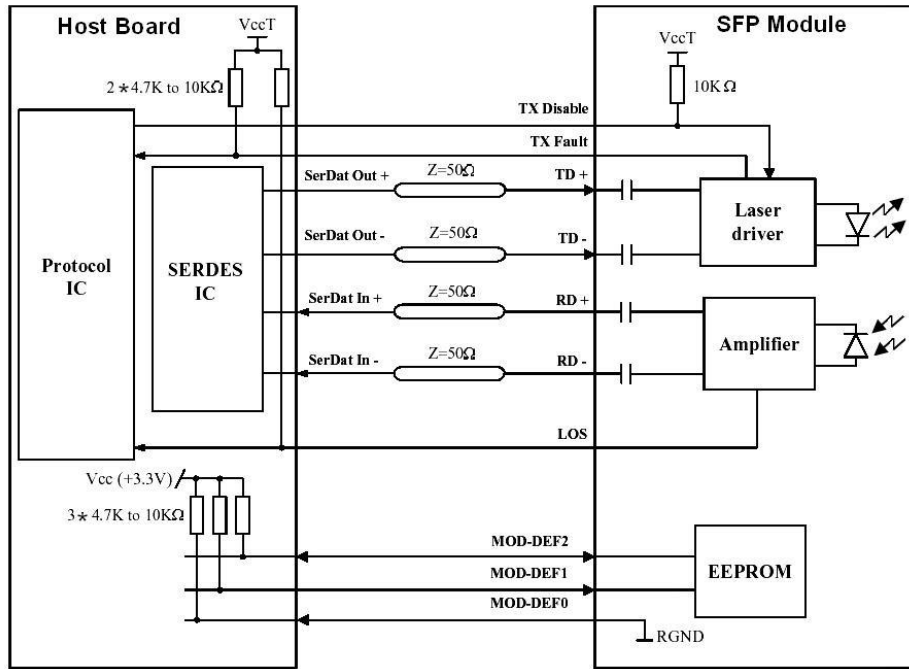
Recommended High-speed Interface Circuit
