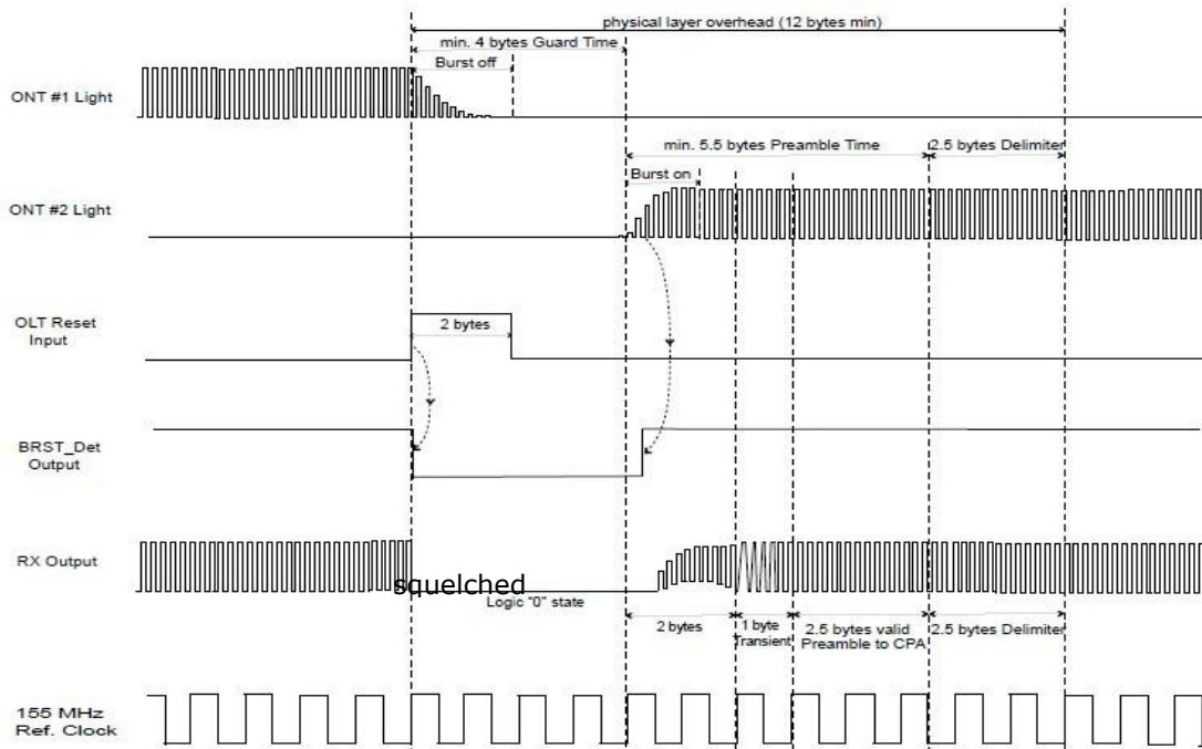
Figure1 Time parameter definition in GPON system
