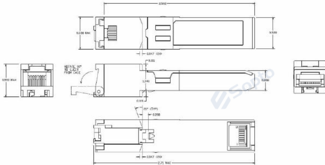
Figure2. SPT-PTTX-RS1 mechanical dimensions
