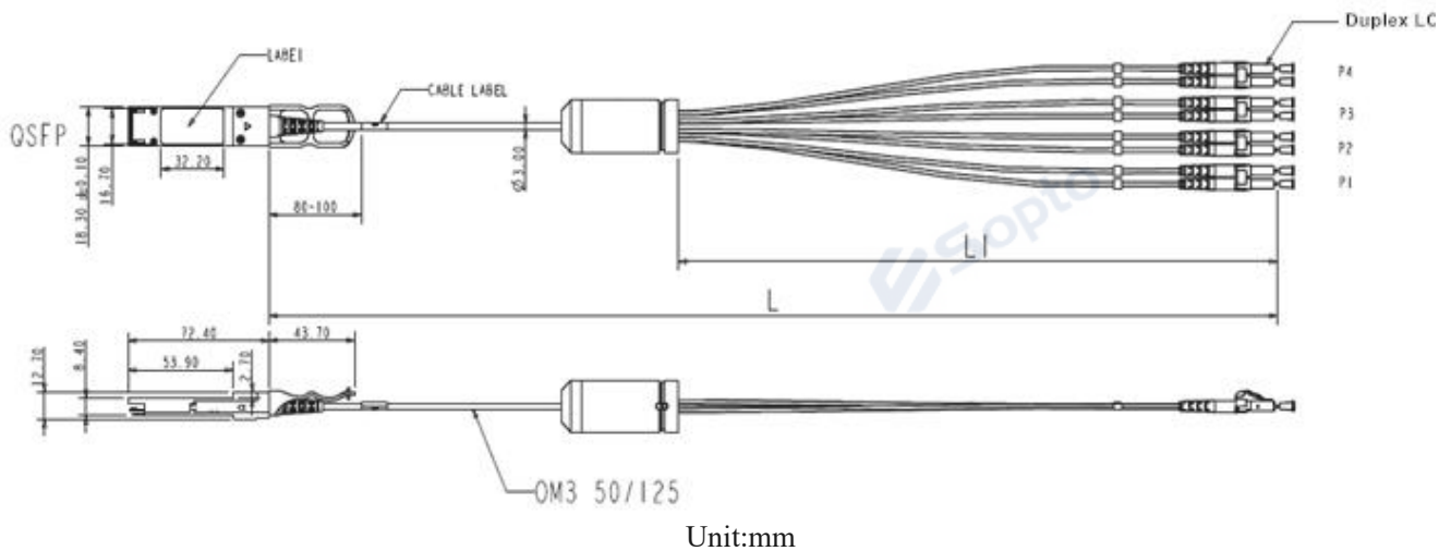
Figure9. Mechanical Specifications
