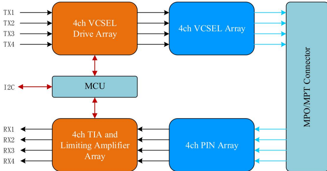
Figure1: Block Diagram
