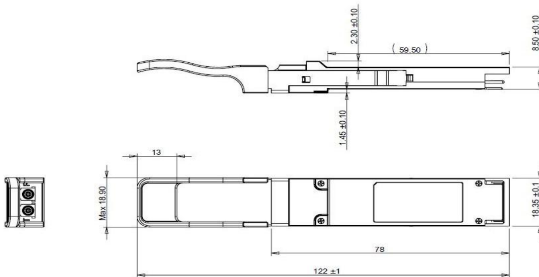
Figure 4. Mechanical Outline
