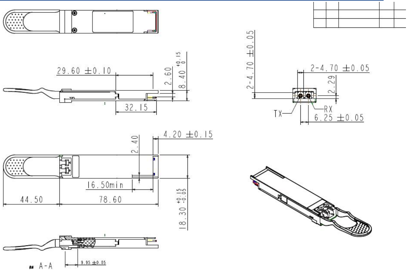
Figure 9. Mechanical Specifications
